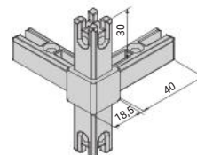
2240075 Corner joint, 4-sided
