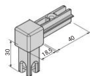
2240073 Corner joint, 2-sided
