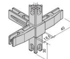
2240077 Corner joint, 5-sided
