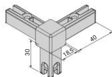
2240074 Corner joint, 3-sided
