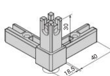
2240083 Corner joint, 3-sided, with adjustable foot
