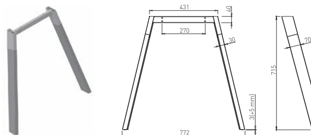
Noga model Wood FE Ø70x30/800
