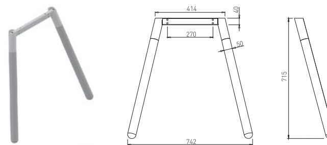
Noga model Wood FE Ø50/800
