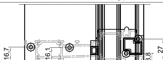
Obrada profila FT-1100F Processing profile FT-1100F
