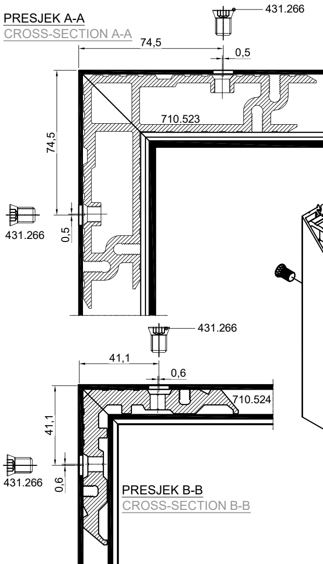
SPAJANJE PROFILA FT-0194F KUTNICIMA CONNECTION PROFILE FT-0194F WITH CORNER BRACKETS
