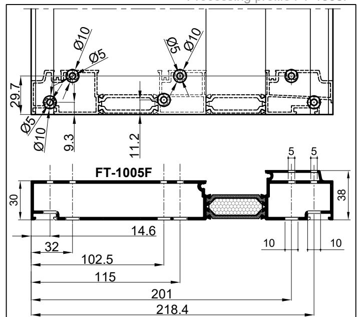
Obrada profila FT-1005F Processing profile FT-1005F
