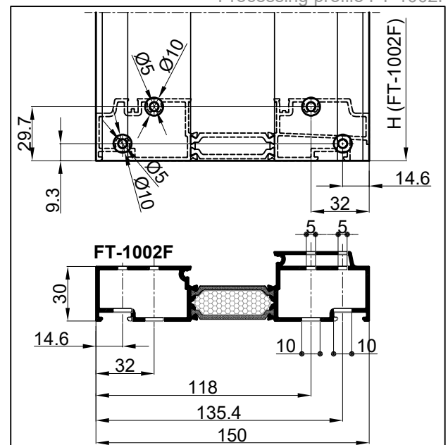
Obrada profila FT-1002F Processing profile FT-1002F
