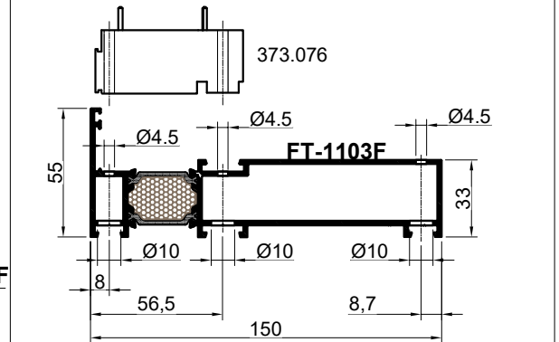
Detalj „1“ Obrada profila FT-1103F Profile processing FT-1103F
