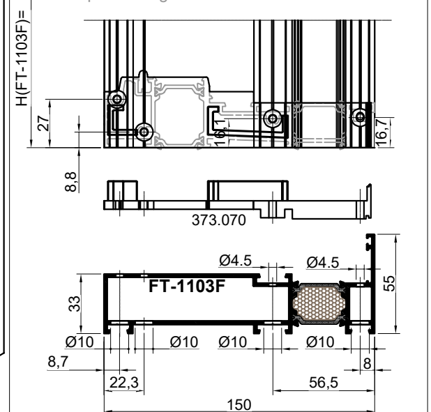
Obrada profila FT-1103F Profile processing FT-1103F
