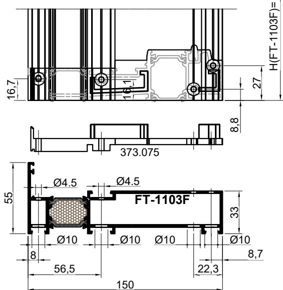
Detalj „2” Obrada profila FT-1103F Profile processing FT-1103F
