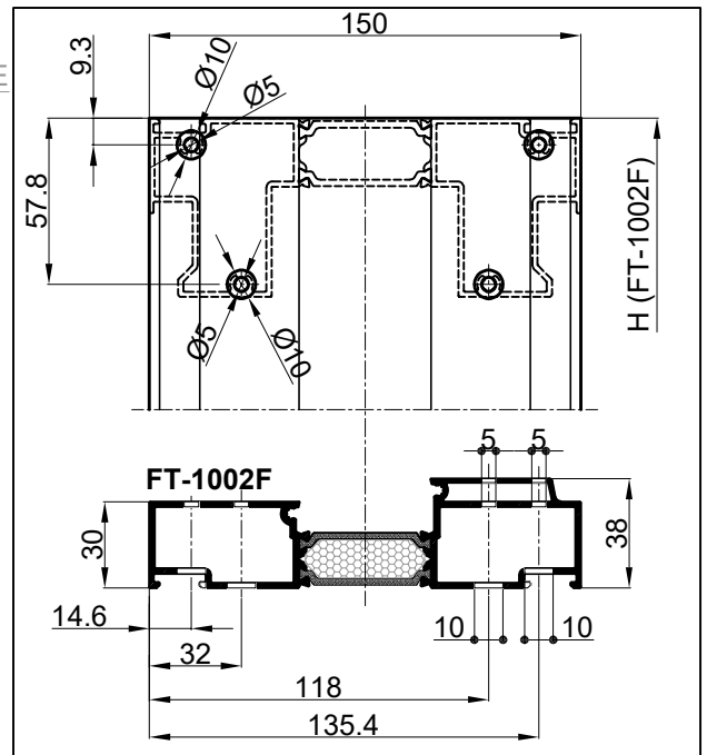
Obrada profila FT-1002F Processing profile FT-1002F
