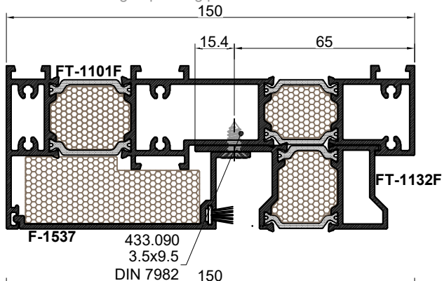
M 1.5:1 presjek kroz otvarajući dio cross section through opening part
