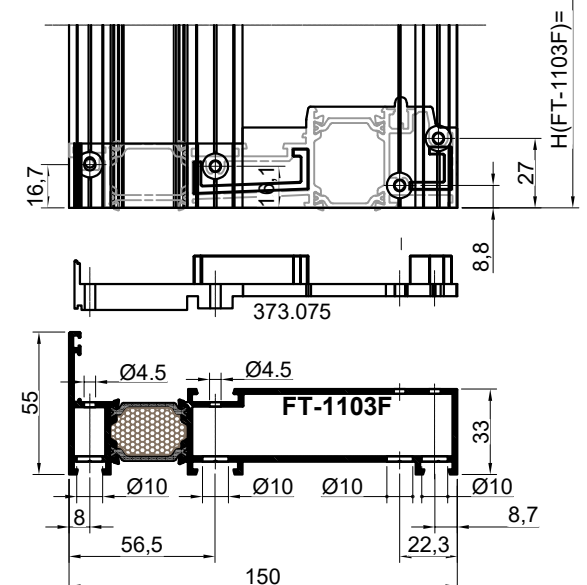
Detalj „2“ Obrada profila FT-1103F Profile processing FT-1103F
