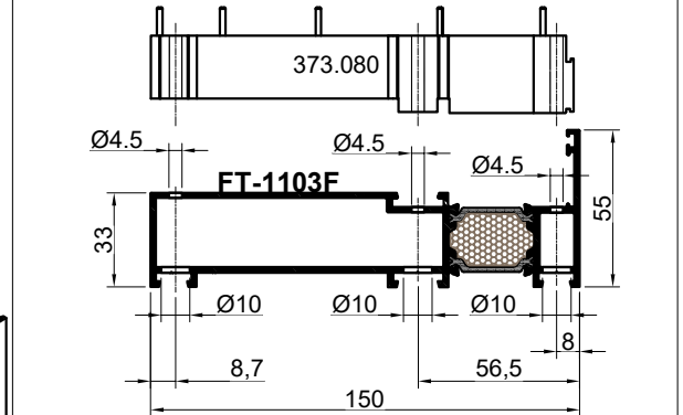
Obrada profila FT-1103F Processing profile FT-1103F
