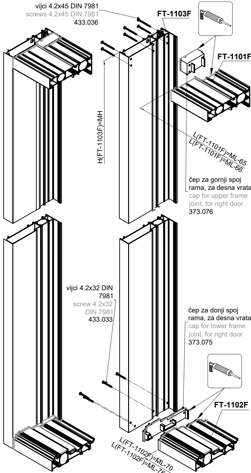
Detalj „1“ Obrada profila FT-1103F Profile processing FT-1103F
