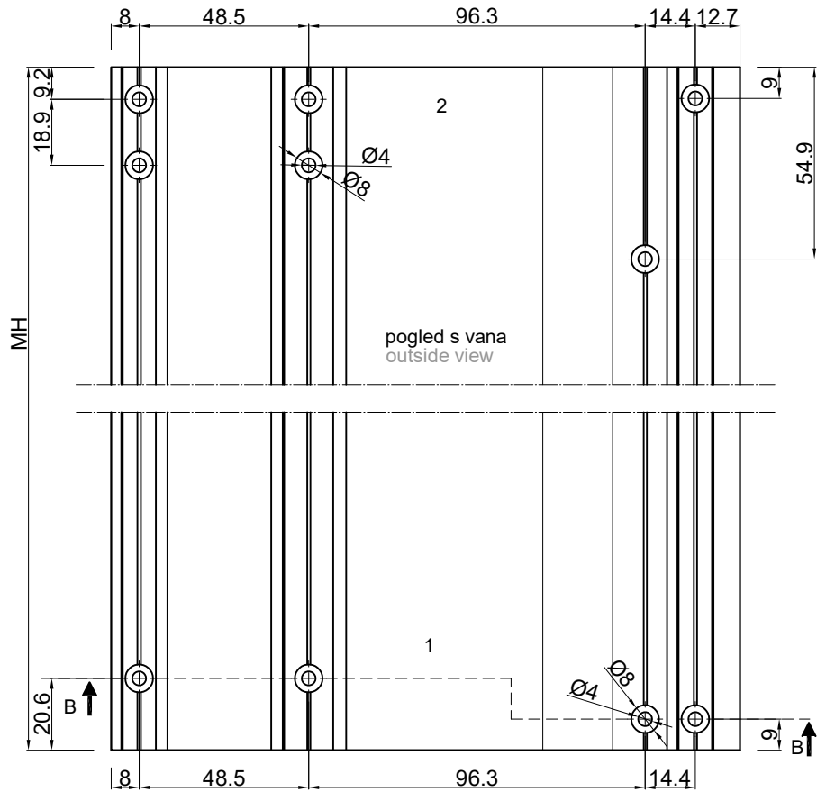
presjek B-B M 1.5:1 cross section B-B M 1.5:1
