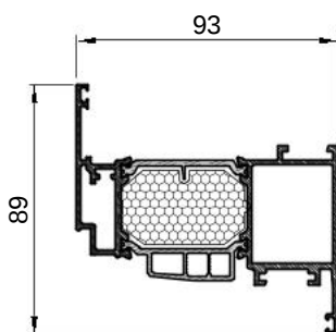
FT-0521F kg/m 1.958
