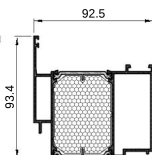
FT-0543F kg/m 2.071
