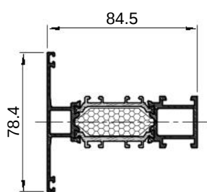
FT-0531F kg/m 1.525
