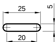
Pogled 1-1 View 1-1
