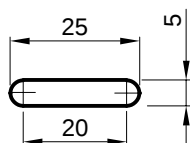
Pogled 1-1 View 1-1
