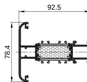
FT-0535F kg/m 1.705
